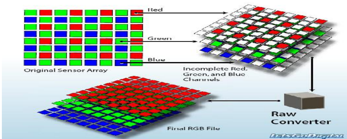
Figure1. Image Enhancement
