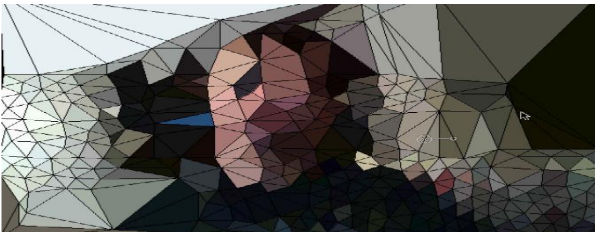
Figure3. linear filtering
