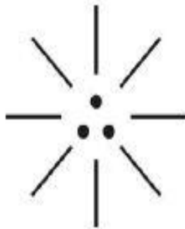
VIRGIN RADIATION (WHITE LIGHT)
