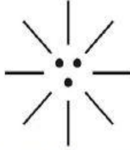
DARK RADIATION (DARK LIGHT)
