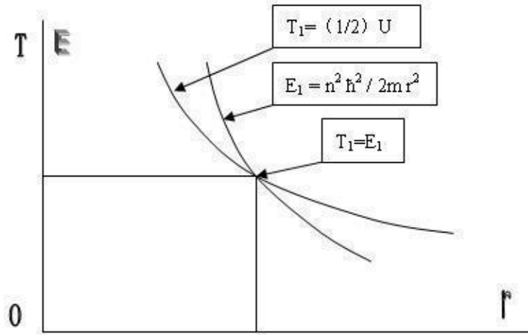
Physical meaning of general equation
