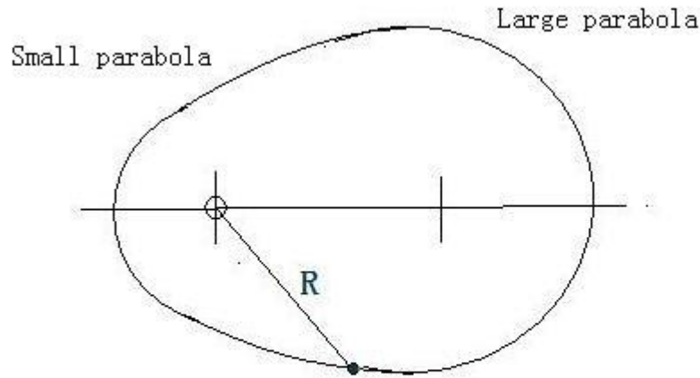
Parabolas of the orbits of heavenly bodies
