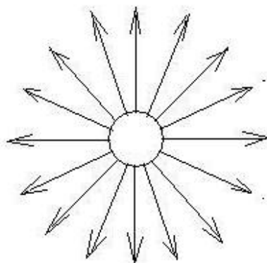
Nuclear radiation energy configuration
