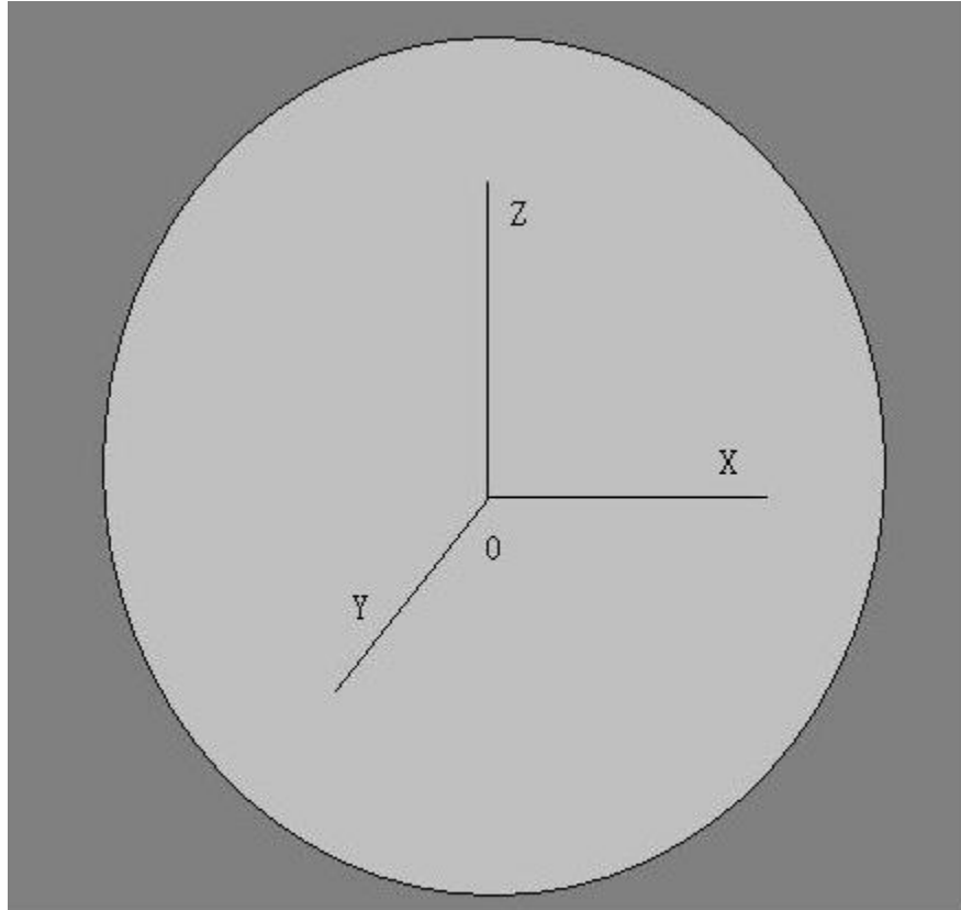
Neutrino universe
