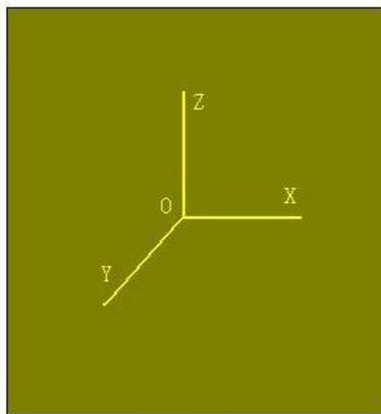
The primitive universe
