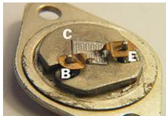
Fig No: 6 Internal parts of transistor 2N3055
