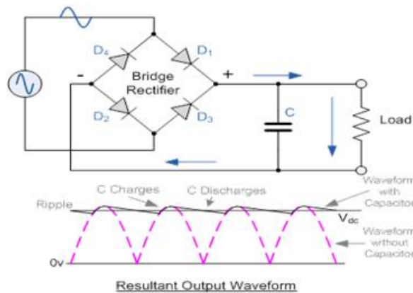
Fig No: 5 Circuit diagram and output waveform of bridge rectifier
