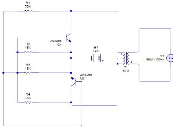
Fig No: 4 Circuit diagram of the inverter
