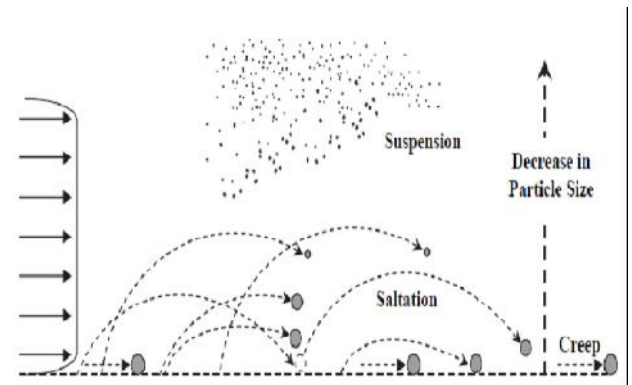
Fig 3: Modes of soil particle transport during wind erosion
